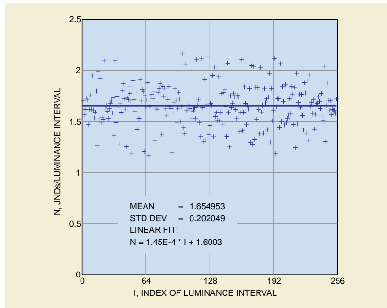
Figure D.1-4. LUM and FIT measures of conformance for a the transformed Display Function of an emissive Display System
