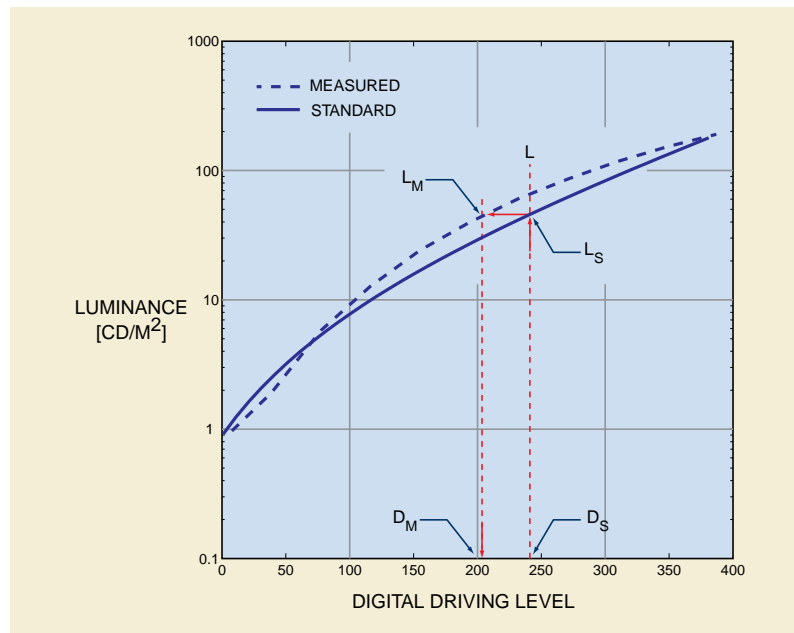
Figure A-1. Illustration for determining the transform that changes the Characteristic Curve of a Display System to a Display Function that approximates the Grayscale Standard Display Function
