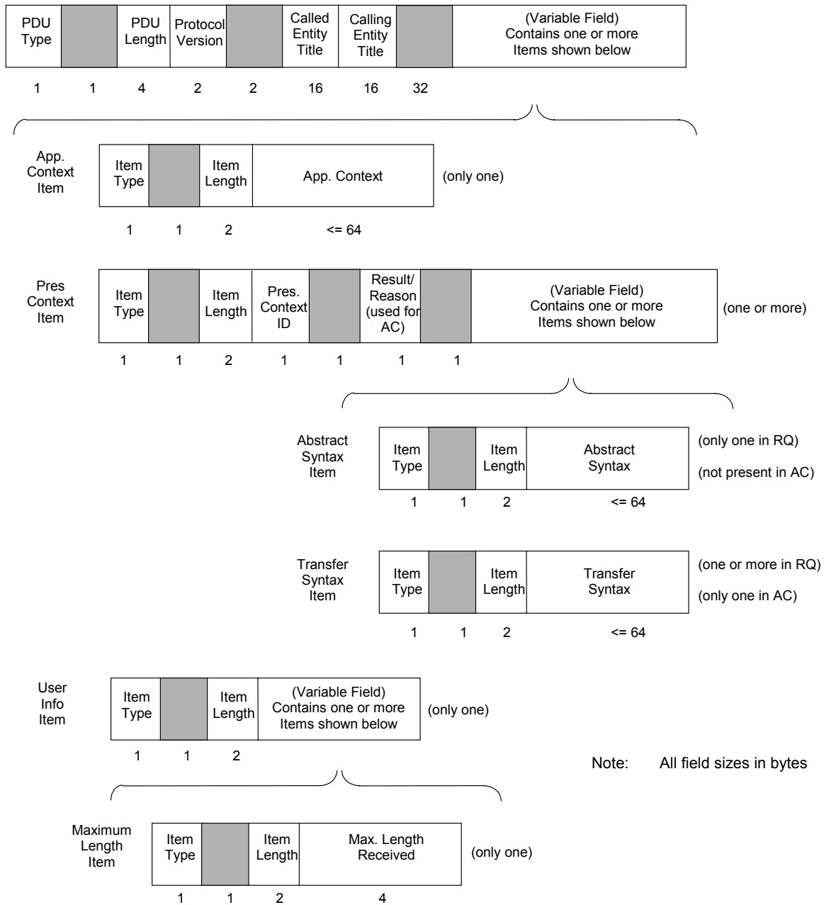
Figure 9-1 PROTOCOL DATA UNITS STRUCTURE AND ENCODING
